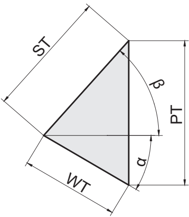
斜楔行程图 Diagram of Cam Travel
